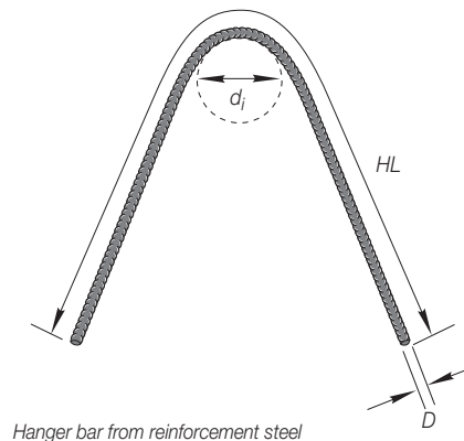
Hanger bar from reinforcement steel
