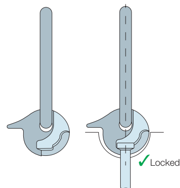
Locking Well interlocks with the Anchor Head
