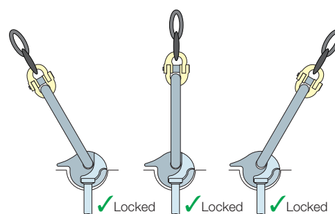
Unique design ensures safe engagement for all load directions
