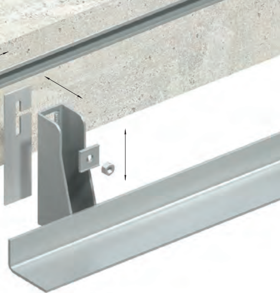
Adjustment of MDC Support System Fixed to Concrete
