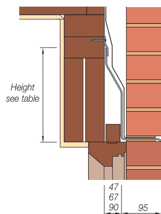
Timber Frame Lintel ST50, 70, 90
