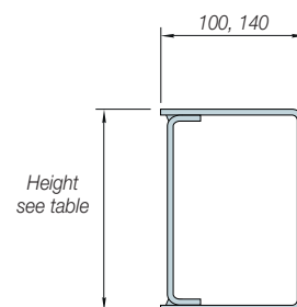
SW Lintels for 100-150mm walls
