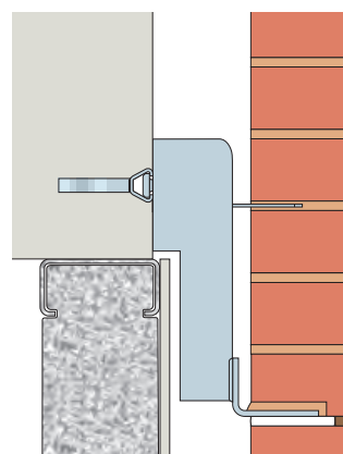
MDC/P/NB Support System
