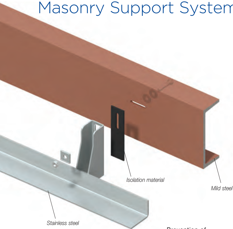
Prevention of Bi-metallic Corrosion
