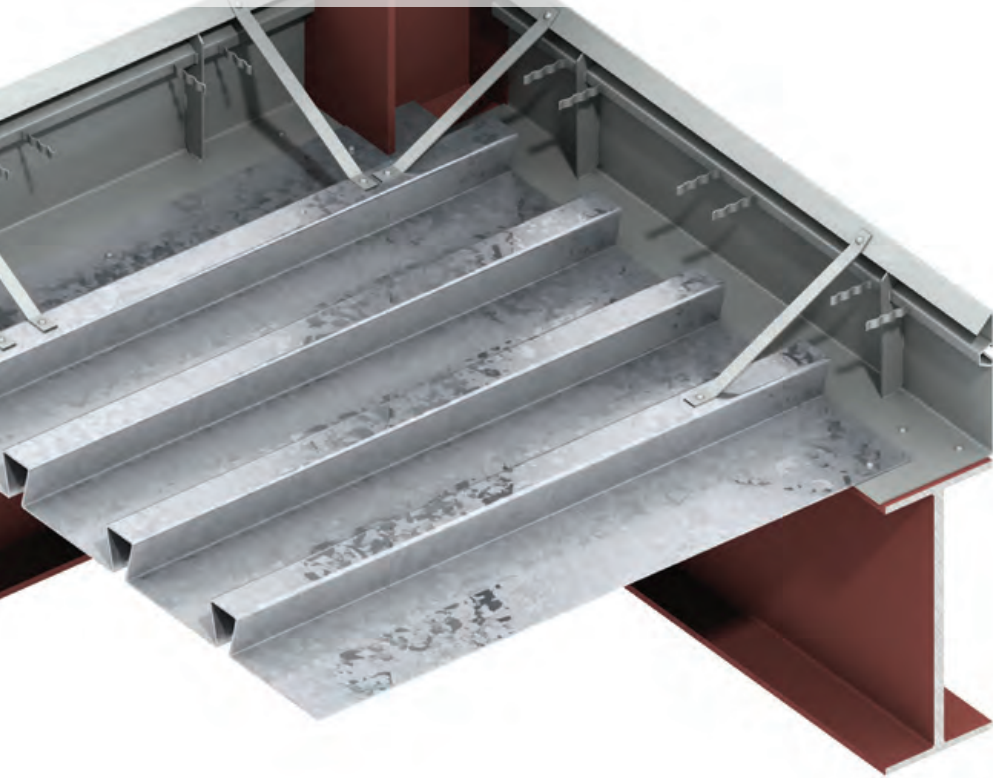
Corner Detail Showing Fixing Straps Between CombiDeck and Metal Deck Shuttering
