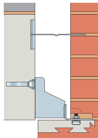
MDC with Precast Masonry Unit
