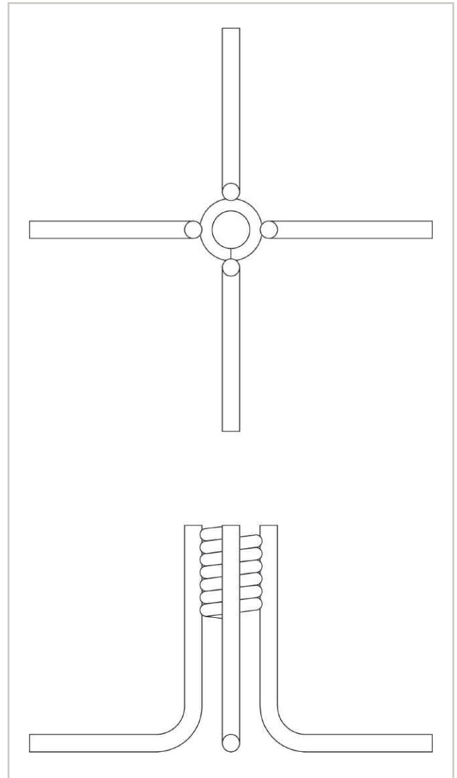
CX-24 COIL LOOP INSERT - DOUBLE FLARED
